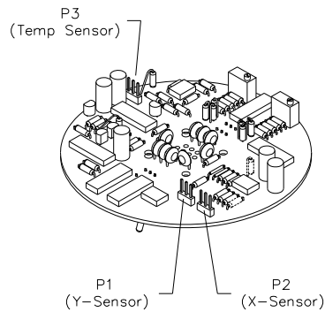
TOP VIEW (Component Side)
