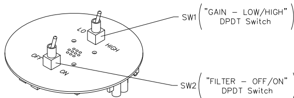
BOTTOM VIEW (Solder/Switch Side)
