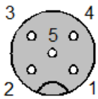
Figure 6: Contact configuration M12 socket
